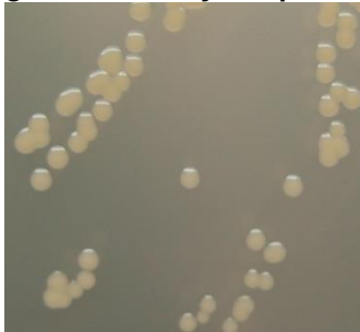
Figure 1: Colony Morphology
